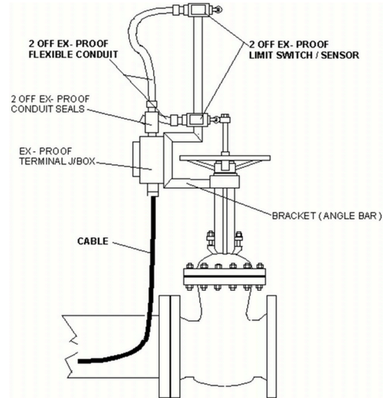
TYPICAL INSTALLATION METHOD BULKY & FLIMSY INSTALLATION
